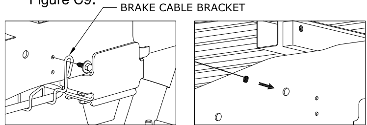
Figure C1: View from outside of Driver Side Frame.
