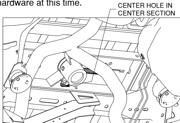
Figure C5: View looking up under truck bed from in front of the axle toward the rear of the truck. (Axle not shown)
