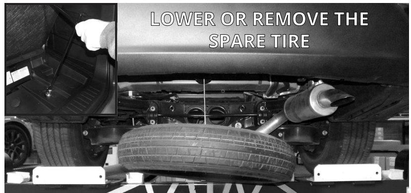
FIGURE A1: VIEW UNDER THE REAR OF THE VEHICLE
