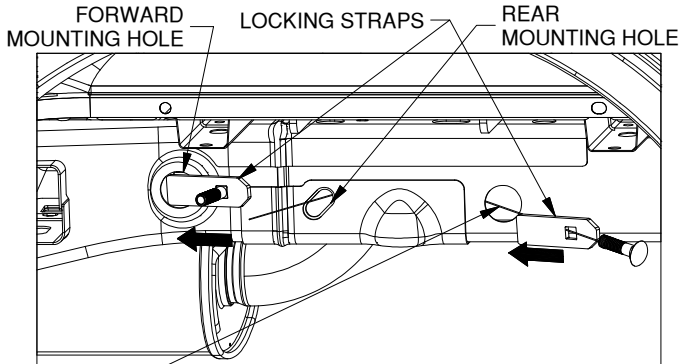
FISH WIRE — Figure C1: View of driver side wheel well.
