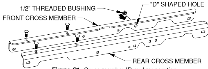
Figure C1: Cross member ID and preparation.
