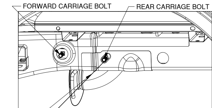
Figure C2: View of driver side wheel well.
