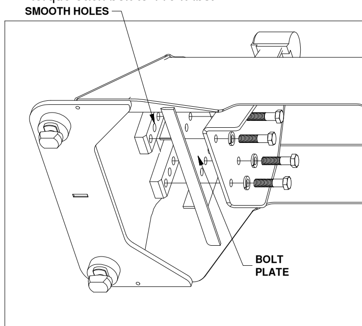
Figure A3: Passenger pivot arm mounting location.
