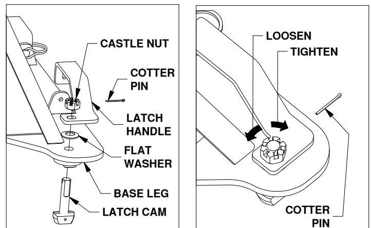
Figure C3: List of latch parts.
