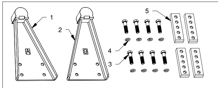
BASE BOLT BAG (RVB3700)
