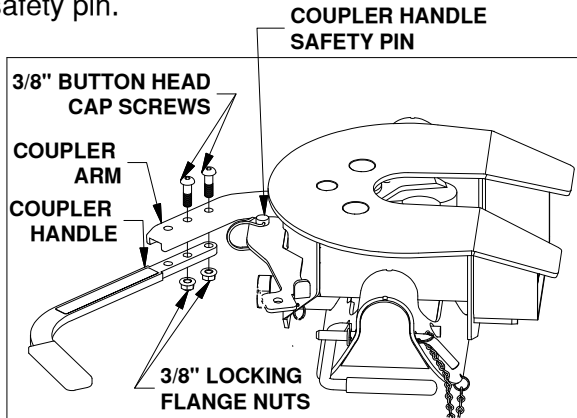
Figure D1: View looking down at side of coupler.
