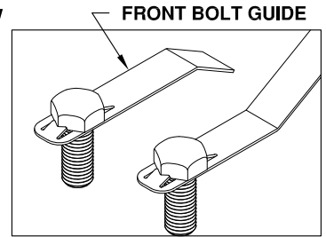
Figure C2: Bolt Guides
