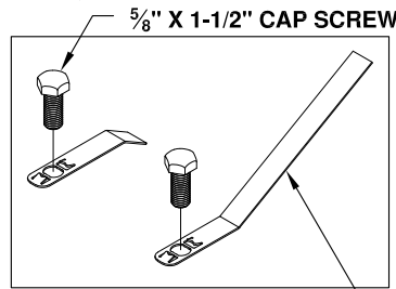
Figure C1: Bolt Guides
