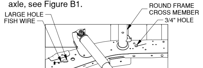
Figure B1: Looking at inside of frame rail.
