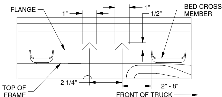
Figure A6: Looking at passenger side wheel well
