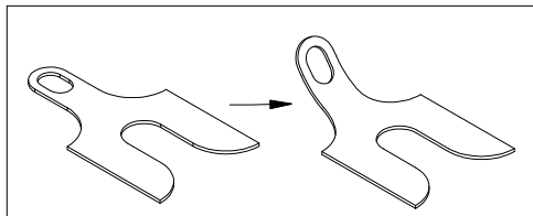
Figure F4: Bolt retainer, before and after.
