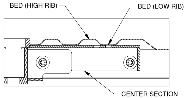
Figure I1: Cutaway view of bed and center section.
