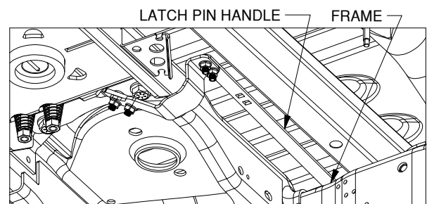
Figure D4: Looking back at driver side of center section.
