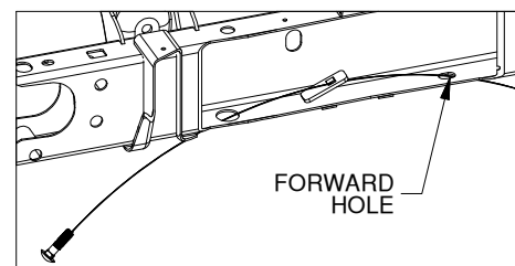
Figures B3 & B4: Cutaway view of the inside of the driver side frame.
