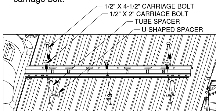
Figure B1: View looking into truck bed from rear of truck.
