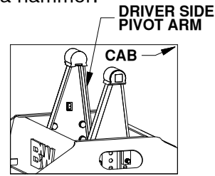
Figure C2: Base view.
