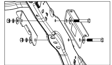
Figure B4: Passenger Side Side plates
