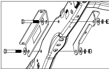
Figure B3: Driver Side Side plates
