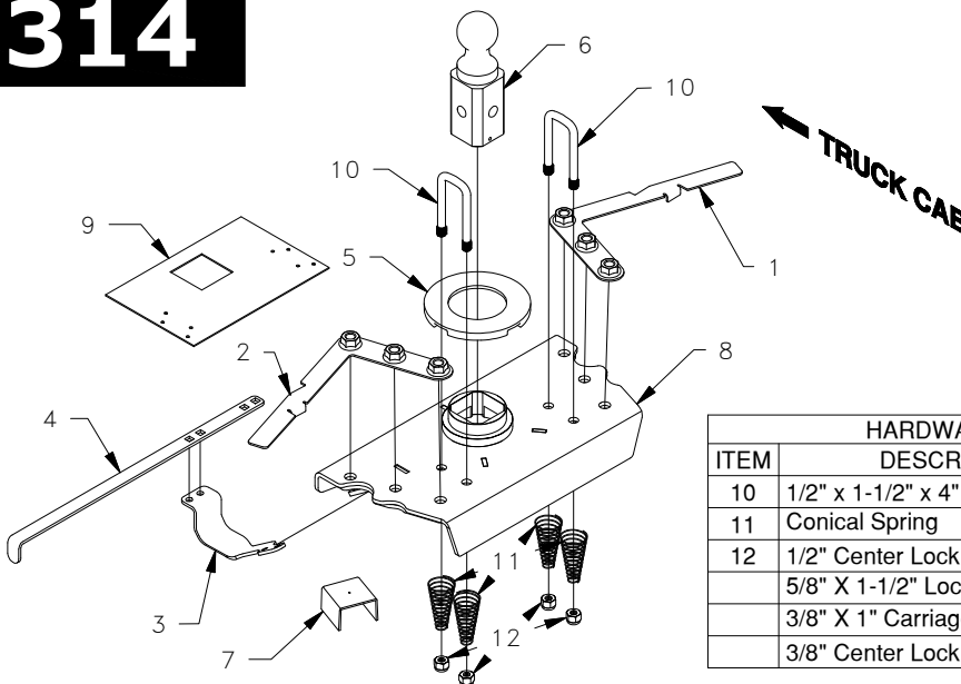
HITCH ASSEMBLY PARTS LIST (GNRK1314)
