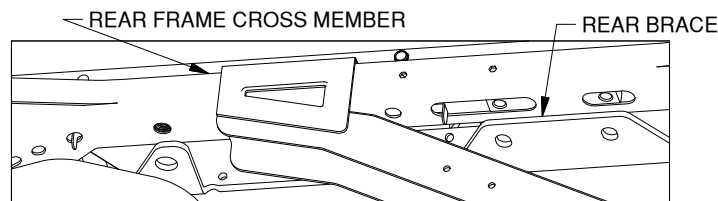
Figures E5: View under bed looking towards the cab.
