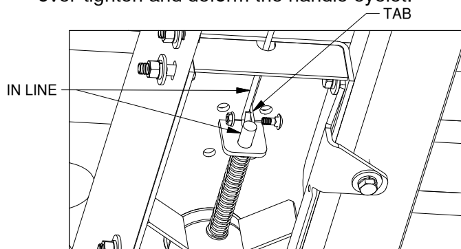
Figure F3: View under driver side of center under the latch pin. (Frame and some hitch components not shown.)
