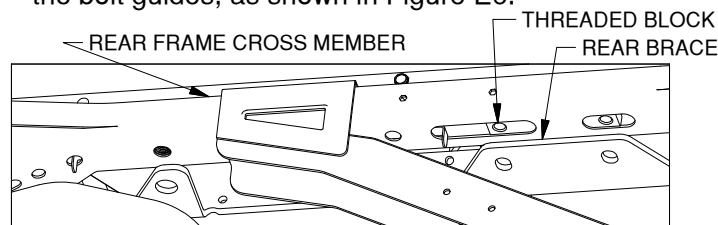
Figures E5: View under bed looking toward the cab.
