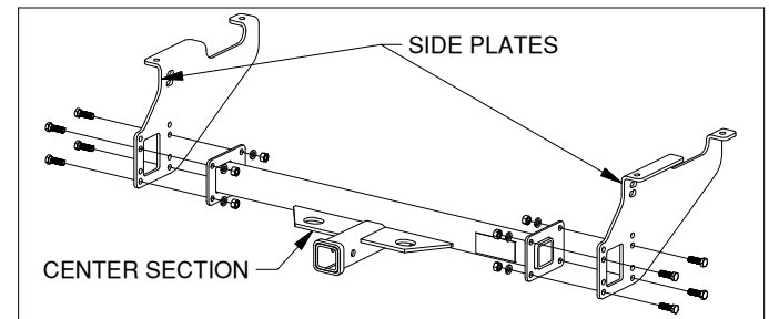
Figure A3: Center section and side plate assembly.
