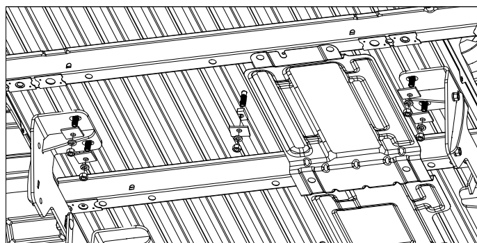
Figure D2: View under bed from rear of truck. (Frame & U-bolts not shown.)
