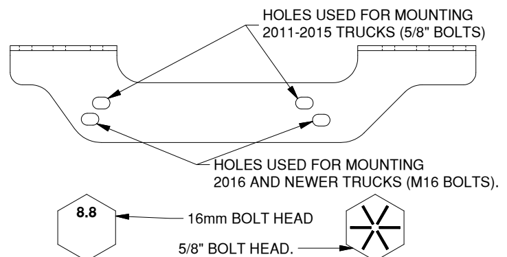
Figure A3: Passenger side plate and bolt head configurations. PAGE 2 of 5
